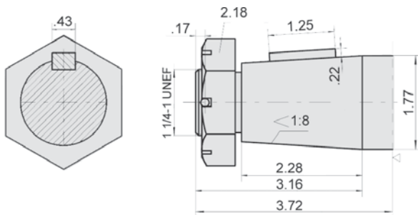
T1 - 1 3/4" Tapered
