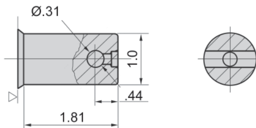
H1 - 1" Parallel .31 Dia. Cross Hole
