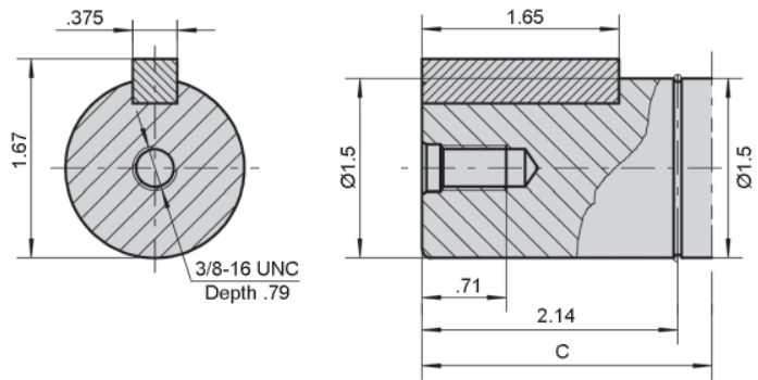
G32 - 1 1/2" Keyed
