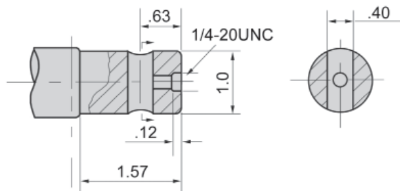
H - 1" Parallel .40 Dia. Cross Hole
