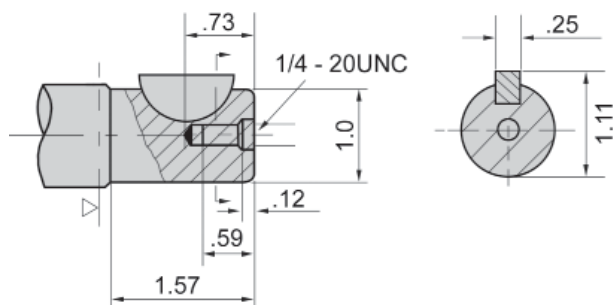
K - 1" Woodruff Key
